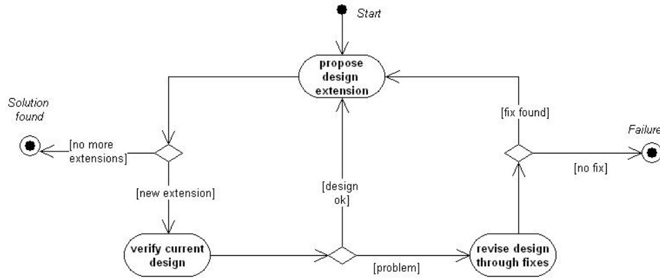
Figure 1.1: Top-level reasoning strategy of the P&R method in the form of a UML activity diagram
