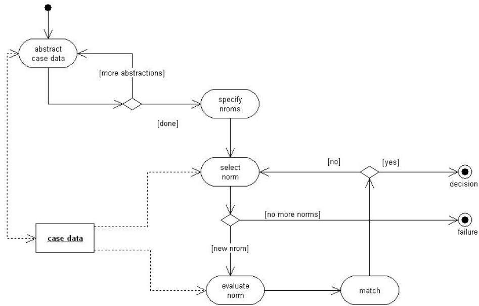
Figure 1.2: Top-level reasoning strategy of the basic assessment method in the form of a UML activity diagram
