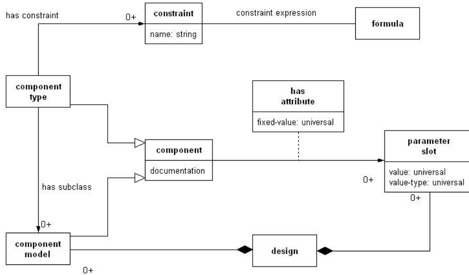
Figure 1.5: Configuration-design ontology in the VT experiment [18] (in the form of a UML class diagram)
