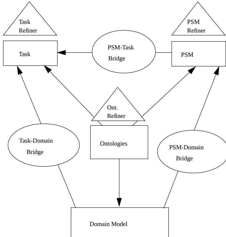
Figure 1. The UPML architecture for knowledge-based system.
