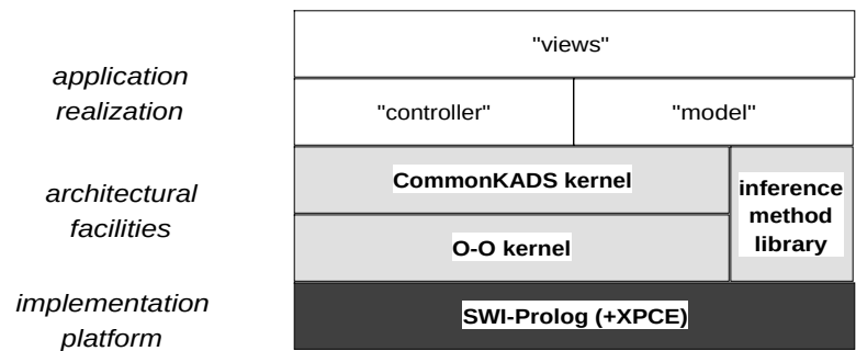
Figure 12.1 Software architecture of the Prolog implementation. The software on top of Prolog can be conceived of as consisting of three layers. The first layer implements object-oriented concepts on top of Prolog and implements the underlying view-update facilities required for the MVC architecture. The second layer implements in a generic way the mapping of CommonKADS objects on the MVC architecture. The third layer is the implementation of the actual application. The inference-method library is an additional architectural facility that provides implementations of algorithms frequently used for realizing inferences, e.g., rule-based reasoning. This library is implemented directly on top of Prolog.
