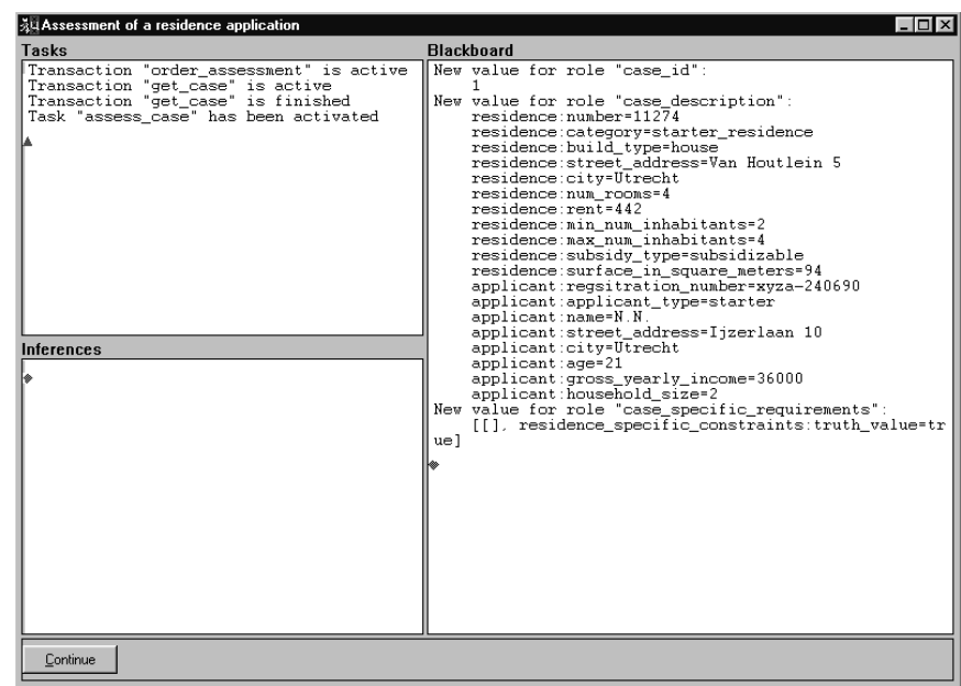
Figure 12.5 Starting the assessment of a residence application. The data of the case to be assessed are shown at the right. For this case, there are no case-specific requirements.
