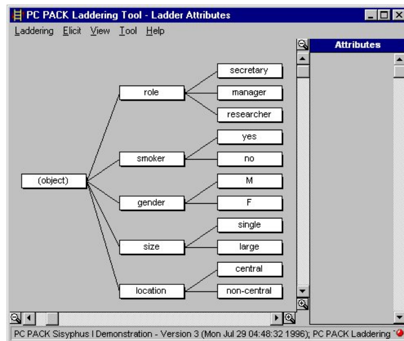
Figure 8.4 A ladder of objects involved in the office-assignment problem.
