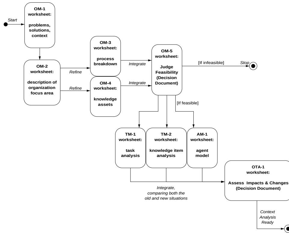
Figure 3.12 A road map for carrying out knowledge-oriented organization and task analysis.
