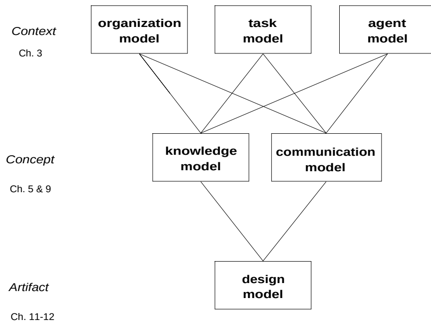
Figure 2.5 The CommonKADS model suite.
